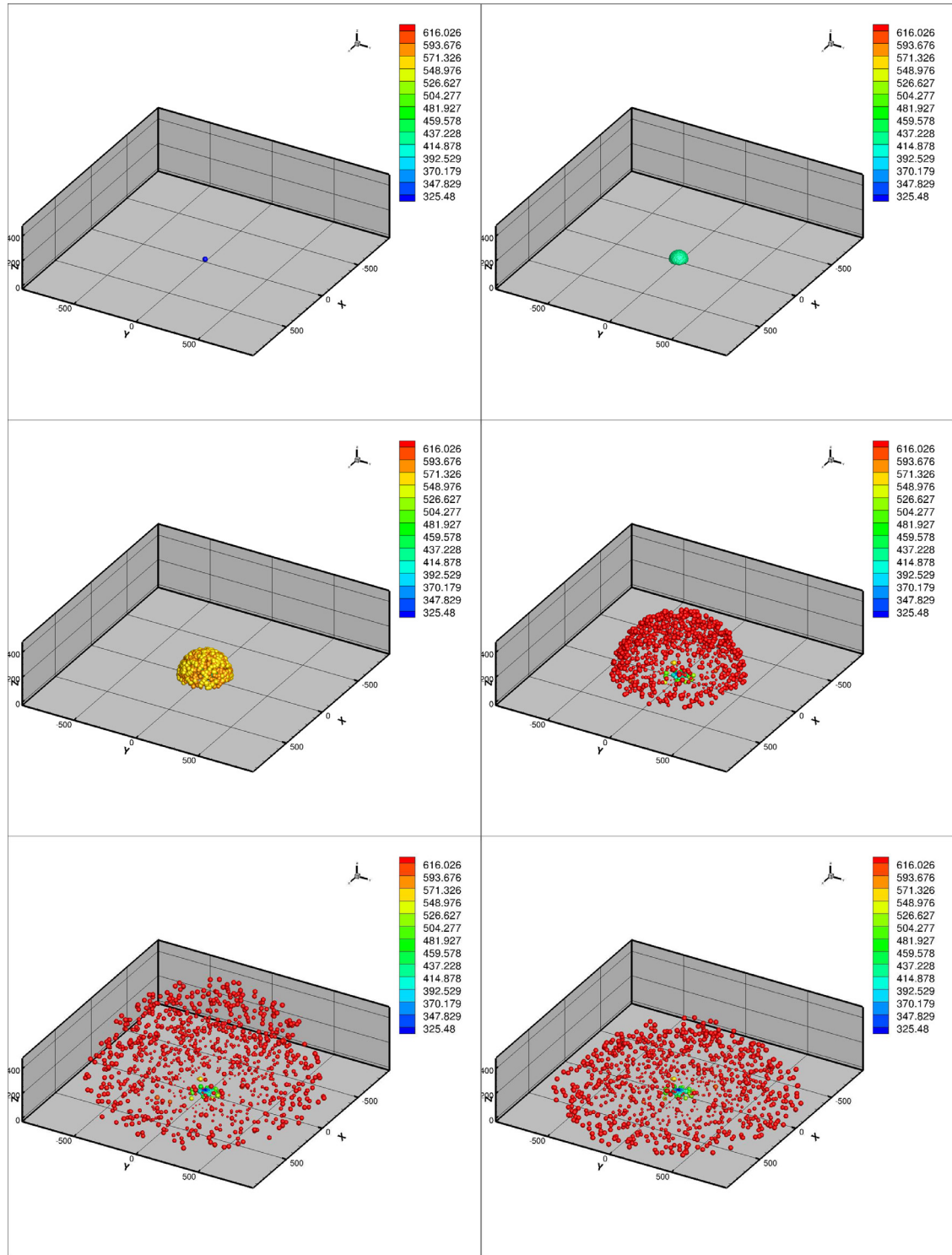
Fig. 6. Case 2: With random fragment masses, m_i = (M/N)(1 + A_i) , where -0.95 \leq A_i \leq 0.95 , with detonation energy, E = 3.6 \text{ kg TNT } E = 16.66 \times 10^6 \text{ J} , with mass of 26.15 kg yielded a blast radius of 784.920 m and a mean temperature of \theta = 174.34 \text{ K} . However, as Fig. 6 clearly indicates material at the core that hits the ground has minimal temperature rise near the blast. The maximum temperature is approximate 615 K. We note that for the case of random fragment masses, we obtained a larger radius for the fragment footprint. We attribute this to more massive fragments are created that are less affected by drag. As a result, a fraction of these fragments travel further. Although this observation could lead to the conclusion that the high drag experienced by aerosol particles would limit their dispersion, these can travel even longer distances. This is possible because aerosols have slow settling velocities and remain suspended for long periods of time. The long suspension times allow them to be carried long distances by ambient wind.
