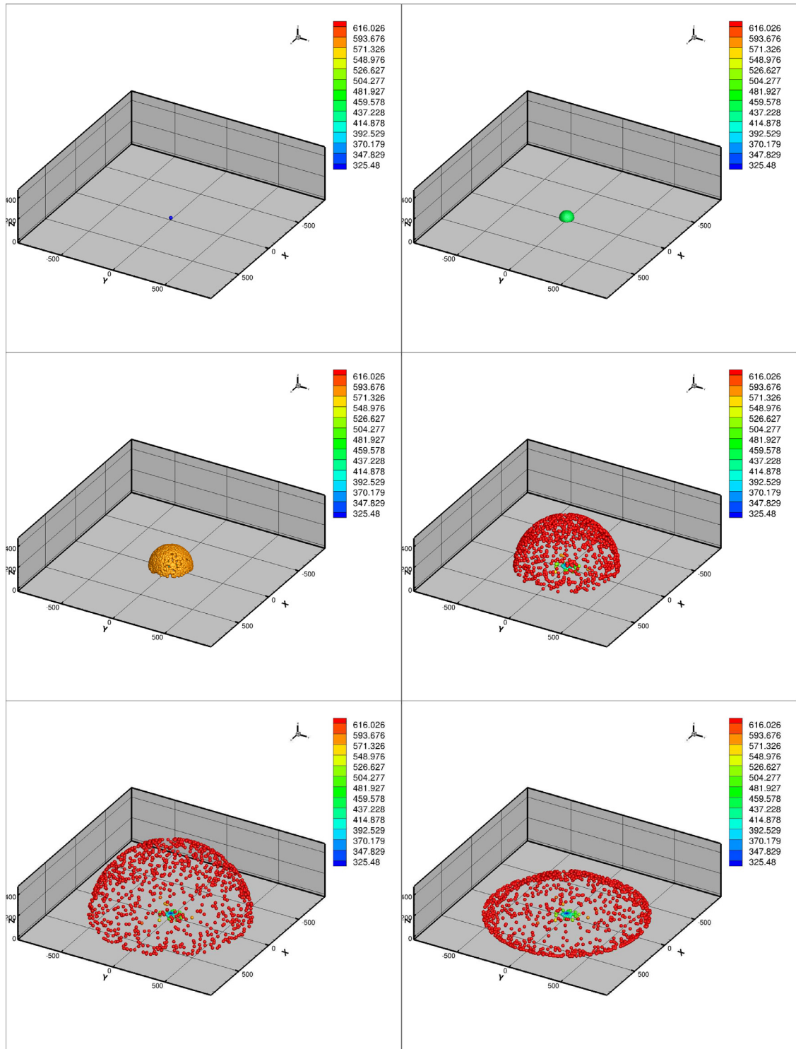
Fig. 5. Case 1: With uniform fragment masses, m_i = M/N . Detonation energy, E = 3.6 \text{ kg TNT } E = 16.66 \times 10^6 \text{ J} , with mass of 26.15 kg yielded a blast radius of 596.278 m and a mean temperature of \theta = 174.87 \text{ K} . However, as the Figure clearly indicates material at the core that hits the ground has minimal temperature rise near the blast. The maximum temperature is approximate 615 K.
