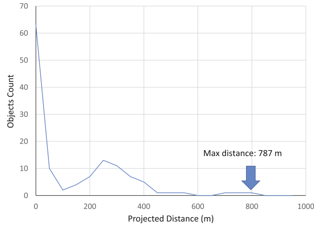
Fig. 4. Histogram of distance distributions.
