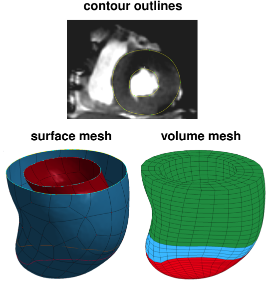
Figure 3: Generation of a patient-specific left ventricular geometry. Two-dimensional magnetic resonance image with contour lines, top, surface representation of the endocardium and epicardium, left, and volume mesh of the left ventricle, right. The finite element mesh consists of 4249 elements, 4296 nodes, and 12888 degrees of freedom for the pre-operative model with distinct infarct region, shown in red, distinct borderzone, shown in blue, and a remote region shown in green.
