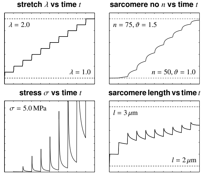
Figure 2: Growth upon uniaxial tension. The stretch is gradually increased from \lambda = 1.0 to \lambda = 2.0 , top left. For each new stretch level \lambda , the stress \sigma increases rapidly and then relaxes as the tissue grows, bottom left. Stress relaxation is caused by a serial deposition of sarcomere units in each cell. The number of sarcomeres increases from n = 50 to n = 75 as the growth multiplier increases from the ungrown state at \vartheta = 1.0 to the growth limit of \vartheta = \vartheta^{\max} = 1.5 , top right. For each new stretch level \lambda , the length of the individual sarcomeres increases rapidly and then relaxes as new sarcomeres are deposited, bottom right.
